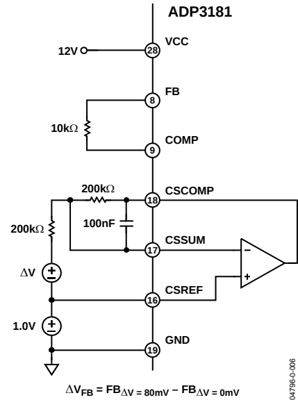
Figure 4. Positioning Voltage
