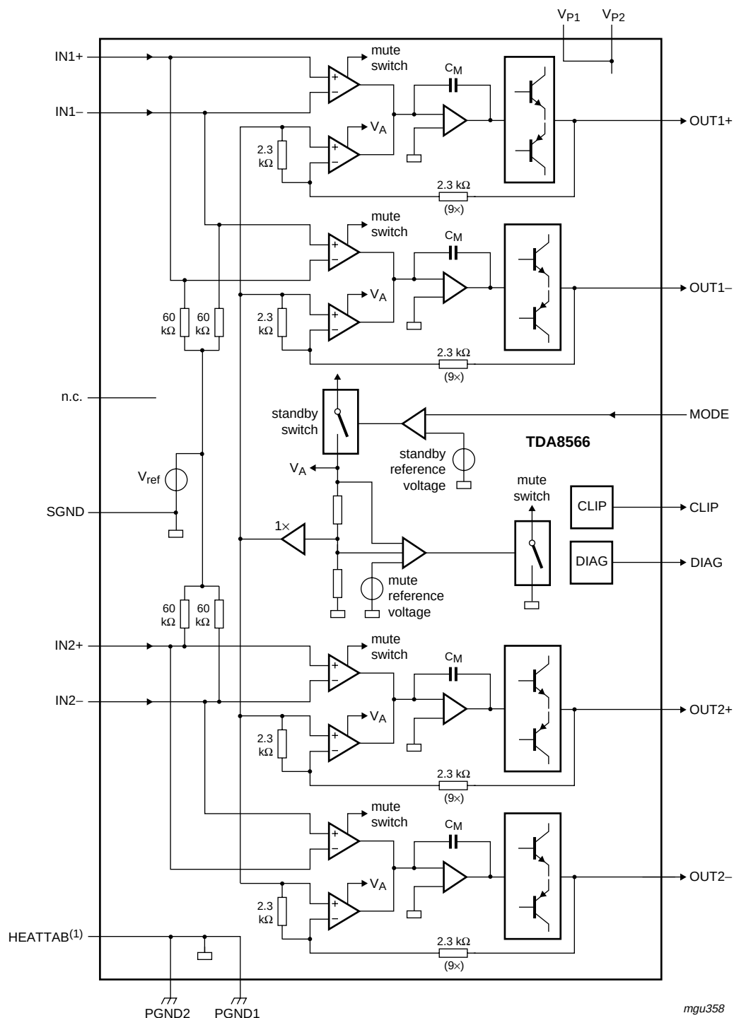
Fig 1. Block diagram
