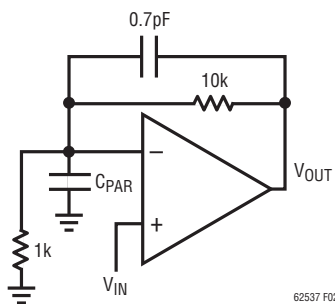
Figure 2. 0.7pF Feedback Cancels Parasitic Pole
