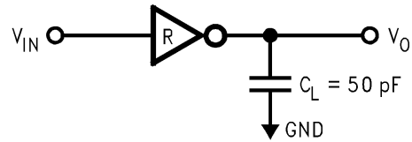
Figure 2. Receiver Load Circuit
