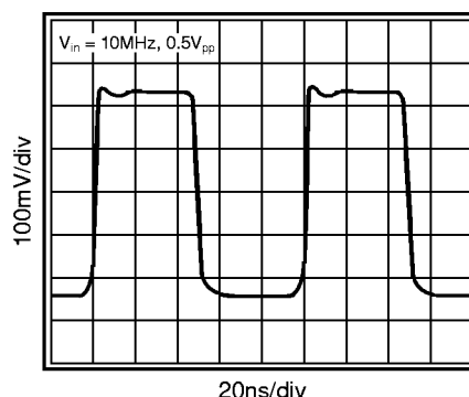
Figure 14: Response After 10m of Cable
