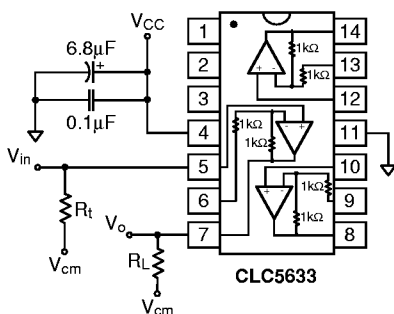
Figure 2: DC Coupled, A_v = +1\text{V/V} Configuration
