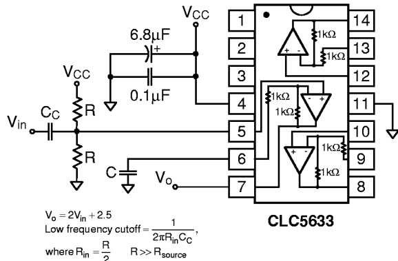
Figure 5: AC Coupled, A_v = +1\text{V/V} Configuration
