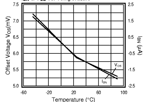
I_{BN} & V_{OS} vs. Temperature
