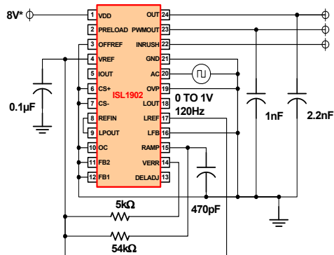
FIGURE 7. RISE/FALL TIME TEST CIRCUIT
