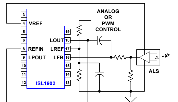
FIGURE 21. USING AN AMBIENT LIGHT SENSOR WITH ANALOG OR PWM INPUT
