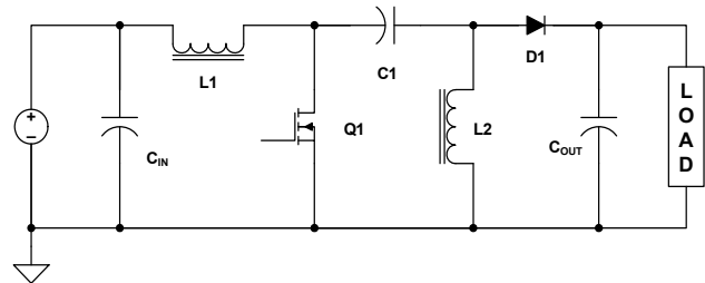
FIGURE 12. SEPIC TOPOLOGY
