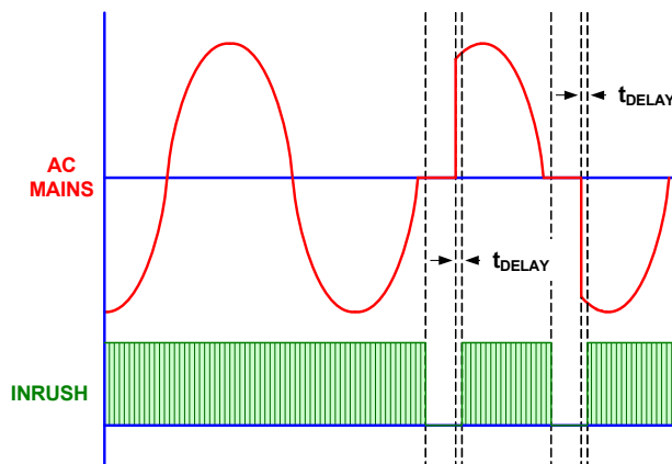
FIGURE 10. AC MAINS TO INRUSH TIMING
