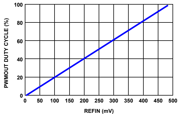
FIGURE 6. PWMOUT DUTY CYCLE vs REFIN
