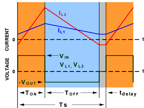
FIGURE 13. SEPIC WAVEFORMS
