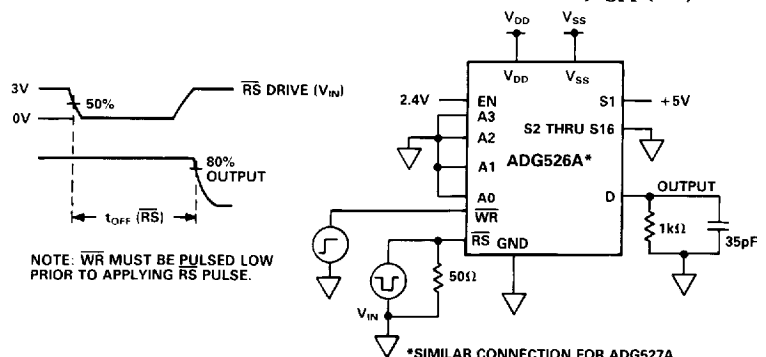
TEST CIRCUIT 10 RESET TURN-OFF TIME, t_{OFF} (RS)
