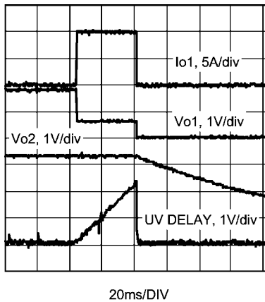
Over-Current and UVP Shutdown ( V_{IN} = 24V , I_{o2} = 0A )
