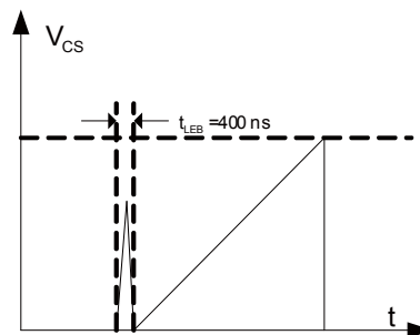
Figure 6: Leading-Edge Blanking
