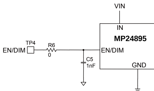
Figure 2: Analog Dimming External Circuit
