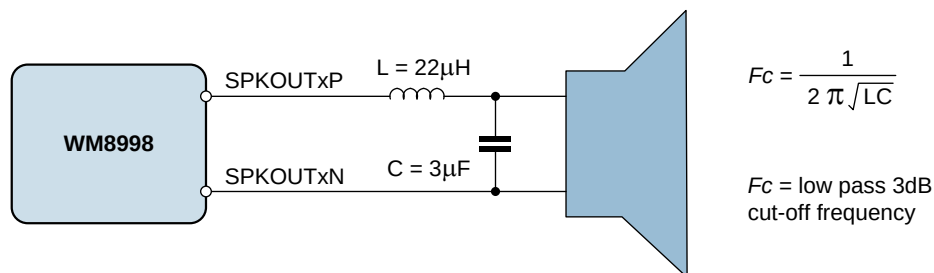
Figure 83 Class D Output Filter Components
