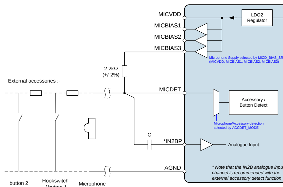
Figure 60 Microphone and Accessory Detect Interface
