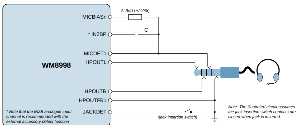
Figure 56 Jack Detect and External Accessory Connections
