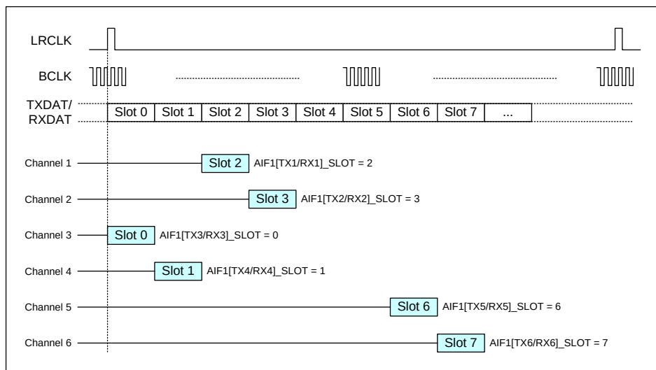
Figure 45 DSP Mode B Example
