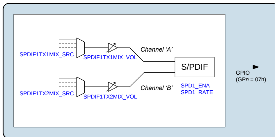
Figure 29 Digital Core S/PDIF Output Generator
