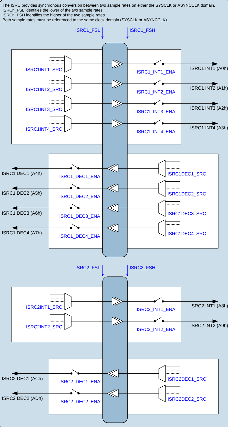
Figure 36 Isochronous Sample Rate Converters (ISRCs)
