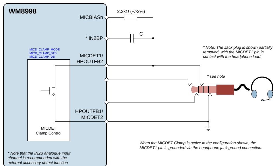
Figure 58 MICDET Clamp circuit
