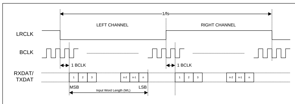
Figure 42 I2S Data Format (assuming n-bit word length)
