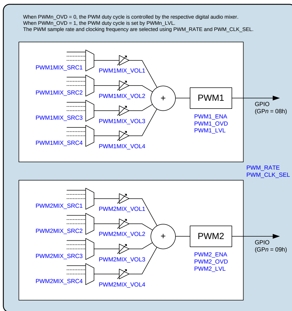
Figure 32 Digital Core Pulse Width Modulation (PWM) Generator
