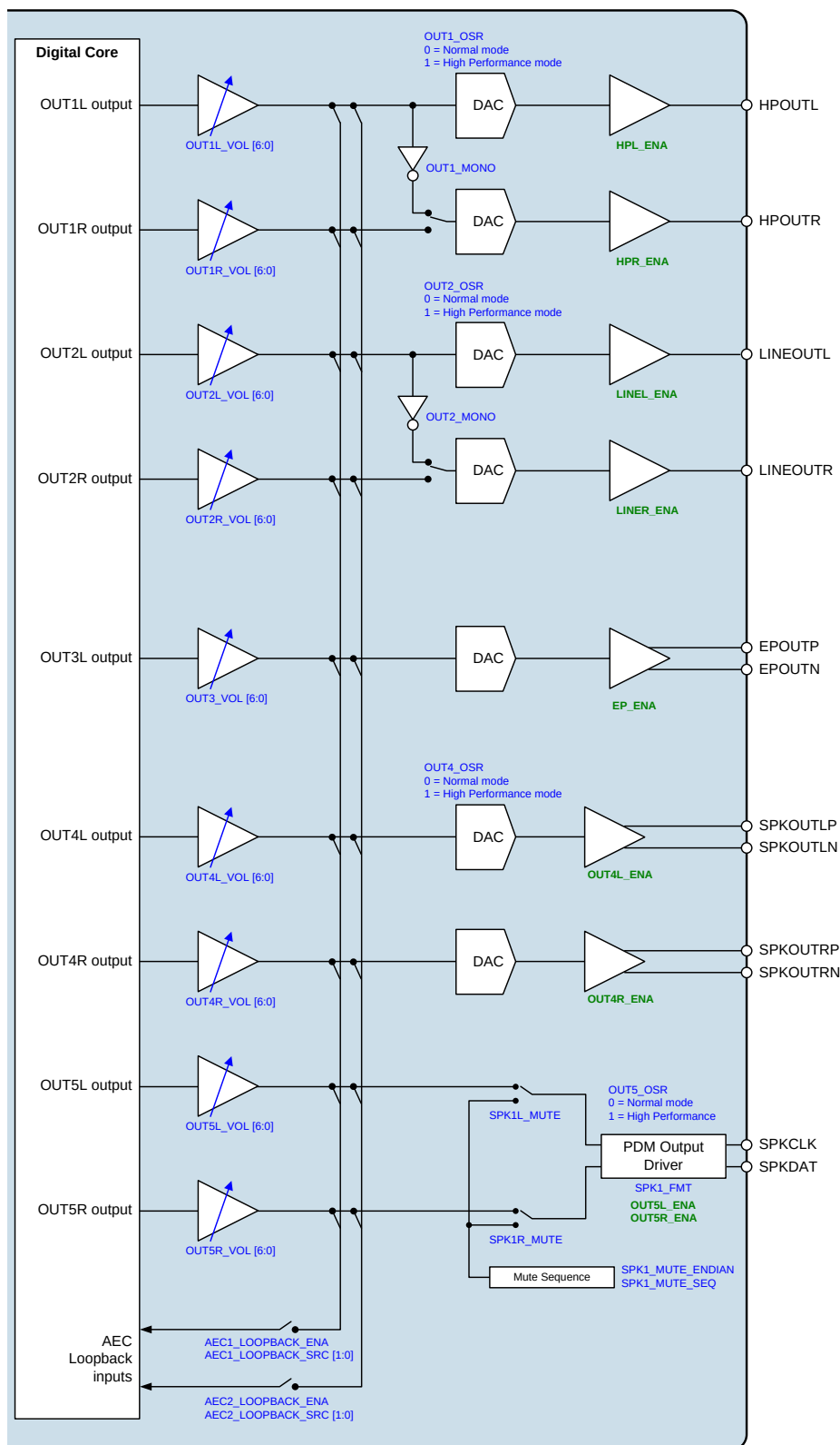
Figure 51 Output Signal Paths
