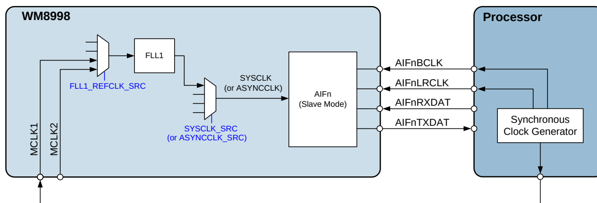
Figure 92 AIF Slave Mode, using MCLK and FLL as Reference
