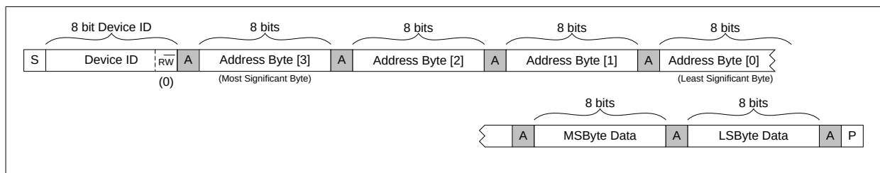
Figure 69 Single Register Write to Specified Address
