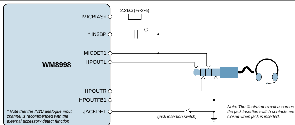
Figure 85 External Accessory Detection
