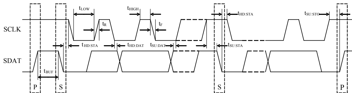
Figure 9.2 SMBus Timing
