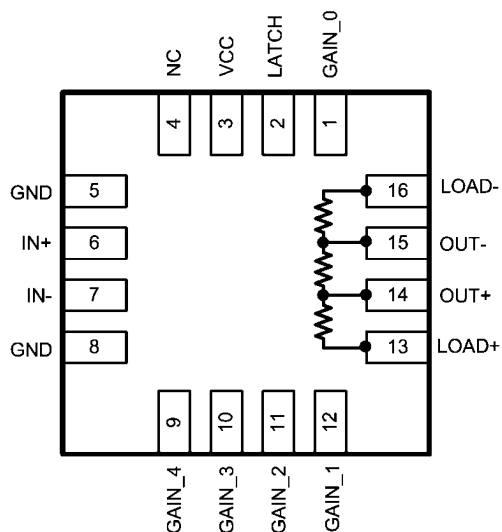
FIGURE 8. Internal Load Resistors
