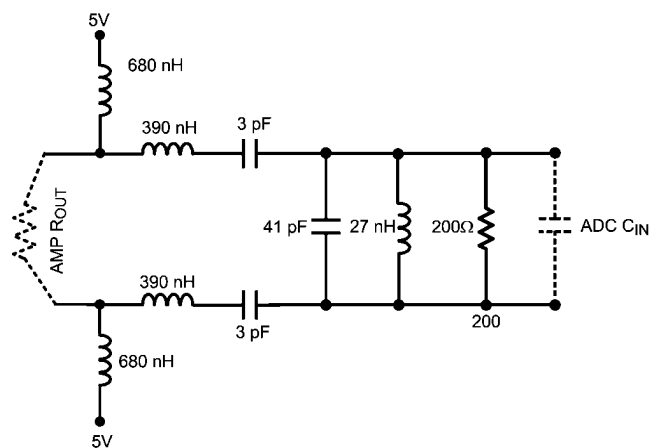
FIGURE 6. Bandpass Filter Center Frequency is 140 MHz with a 20 MHz Bandwidth Designed for 200Ω Impedance
