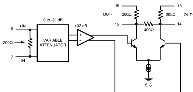
FIGURE 2. LMH6515 Block Diagram
