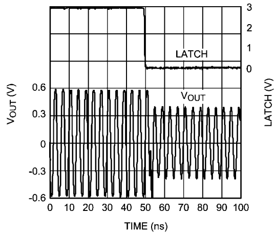
4 dB Gain Step Using Latch Pin
