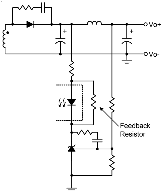
Figure 17. Feedback Resistor
