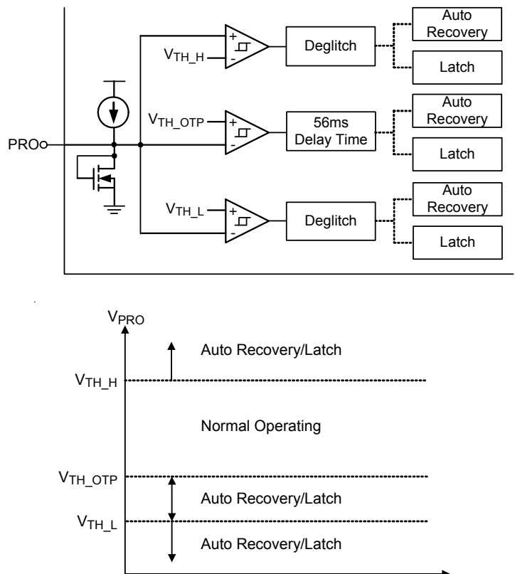
Figure 11. PRO Pin Diagram
