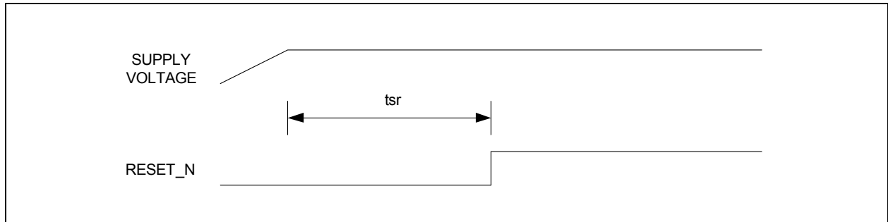
FIGURE 6-7: RESET TIMING
