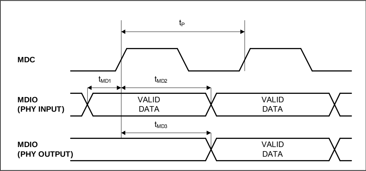
FIGURE 6-6: MDC/MDIO TIMING
