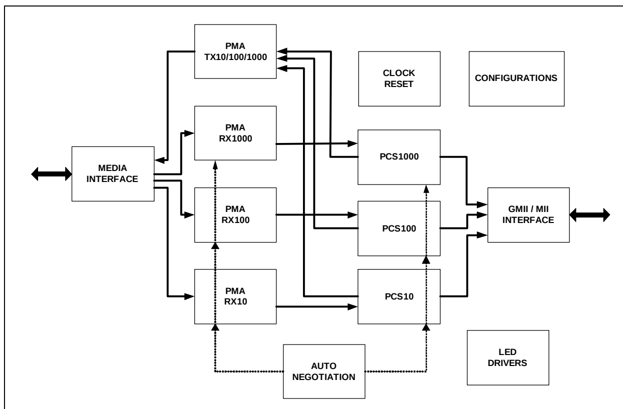
FIGURE 3-1: KSZ9021GQ BLOCK DIAGRAM
