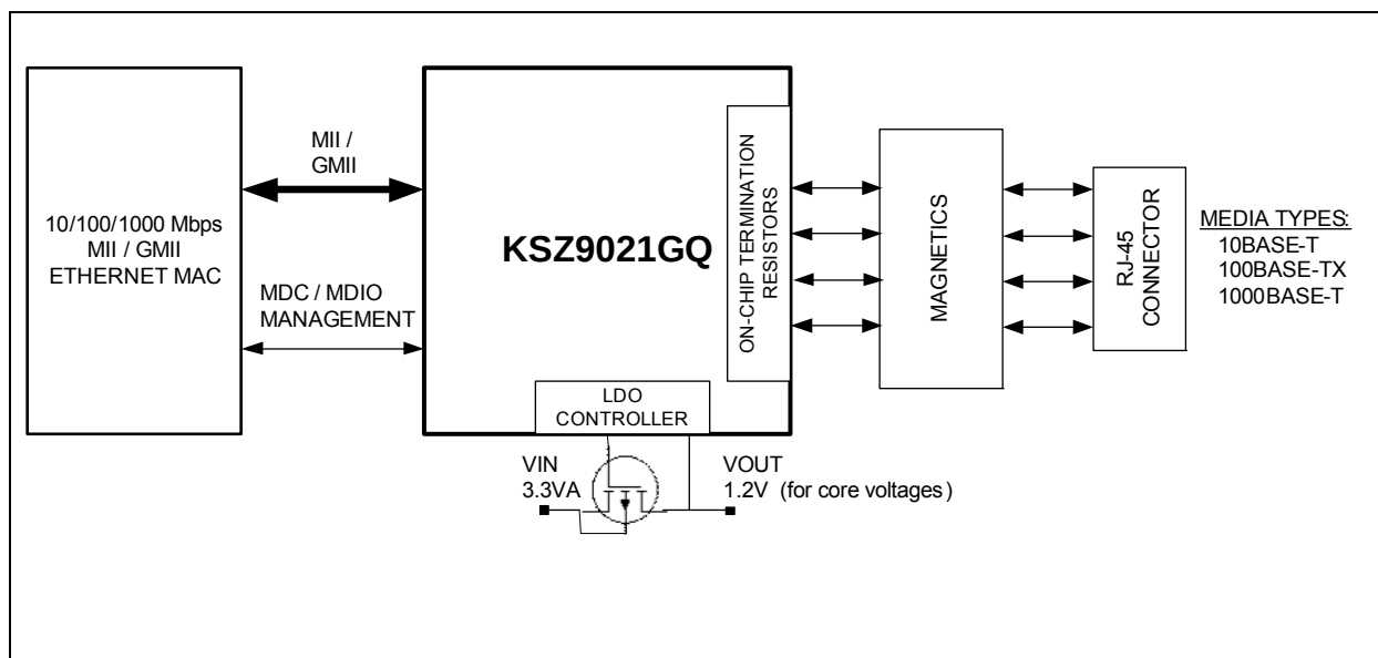
FIGURE 1-1: KSZ9021GQ FUNCTIONAL DIAGRAM
