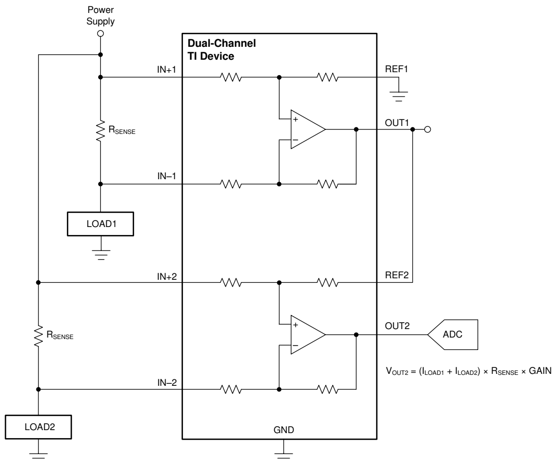
Figure 49. Summing Multiple Currents
