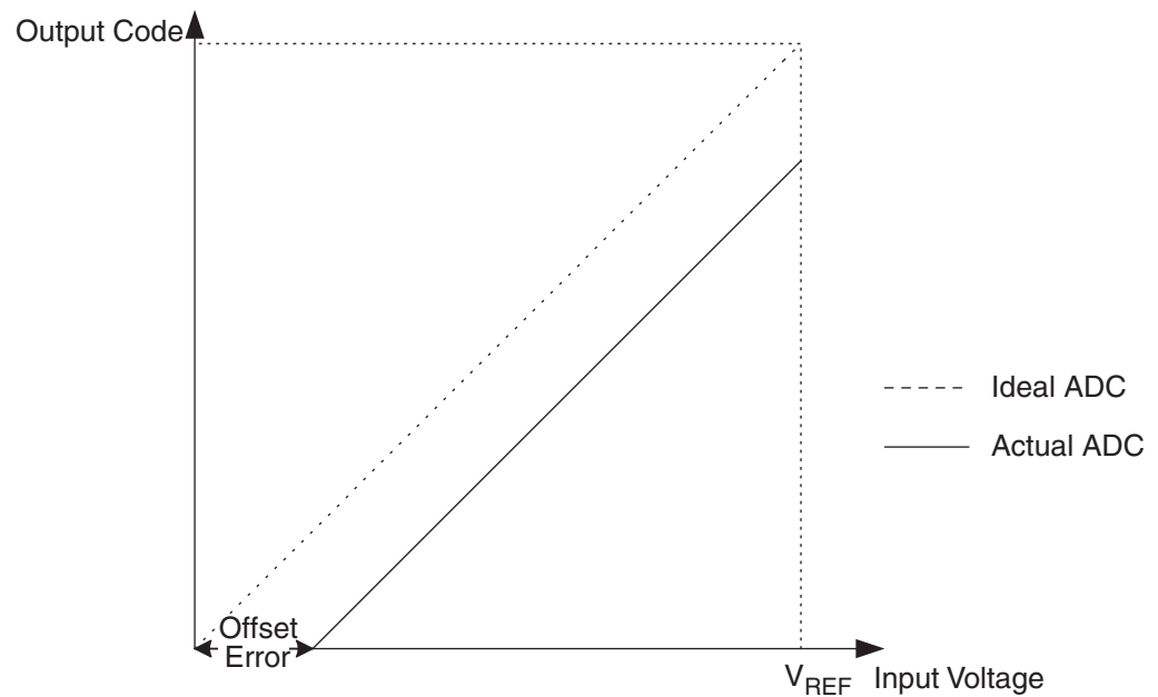
Figure 17-10. Offset Error
