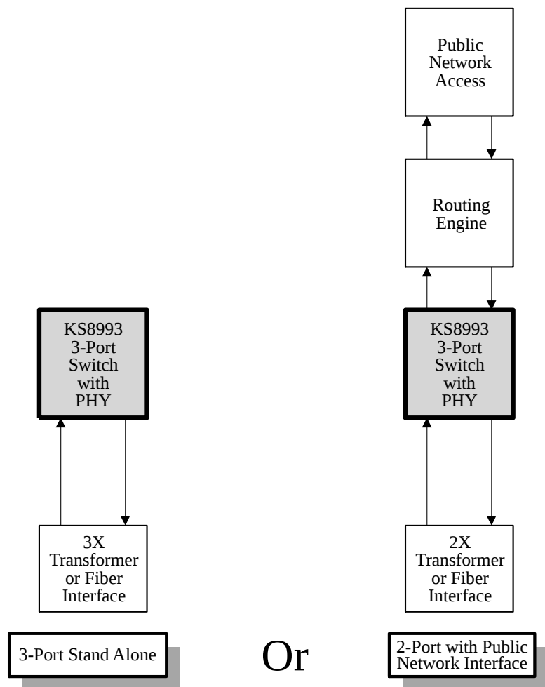
Figure 1. KS8993 Applications
