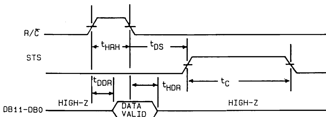
HIGH PULSE FOR R/\bar{C} - OUTPUTS ENABLED WHILE R/\bar{C} HIGH, OTHERWISE HIGH-Z
