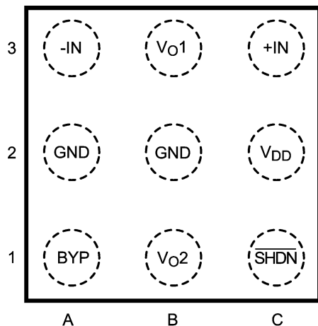
TM Package
