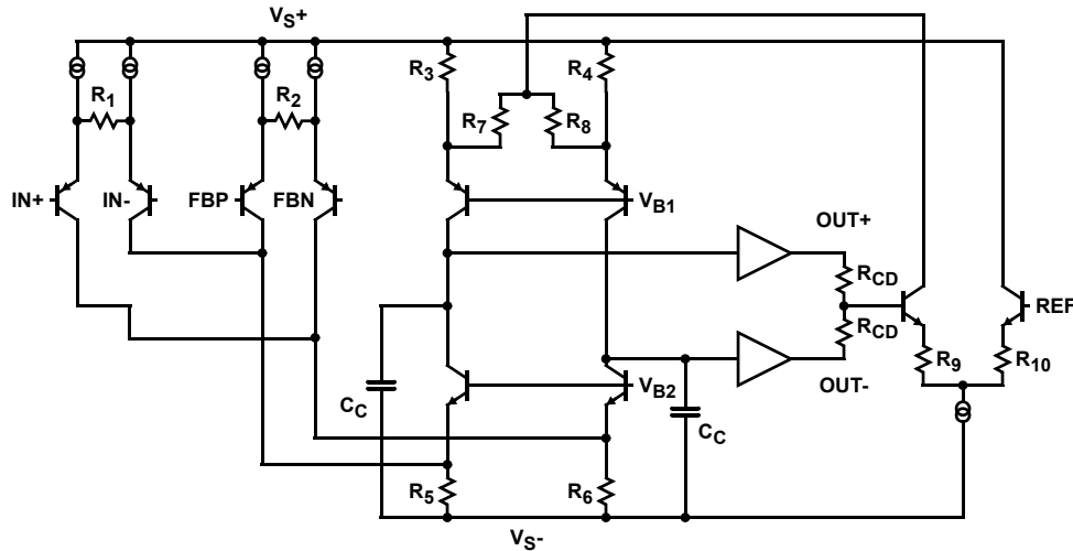
FIGURE 34. SIMPLIFIED SCHEMATIC
