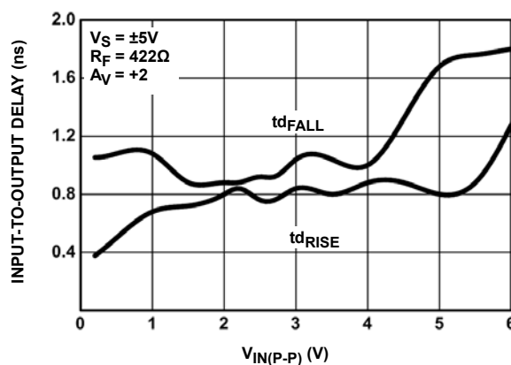
FIGURE 16. INPUT-TO-OUTPUT DELAY
