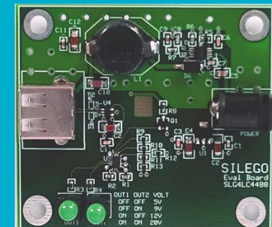
SLG4LC4480 Evaluation Board
