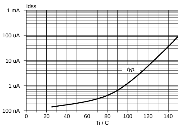
Fig.28. Typical off-state leakage current. I_{DSS} = f(T_J) ; Conditions: V_{DS} = 40\text{ V} ; I_S = 0\text{ V} .
