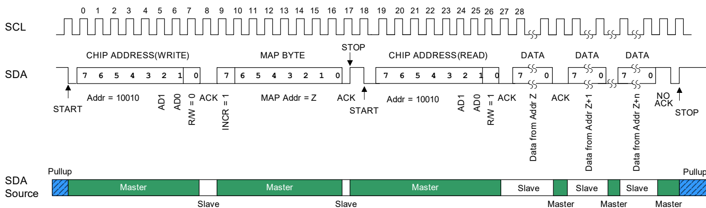
Figure 4-29. Control-Port Timing, I²C Reads with Preamble and Autoincrement
