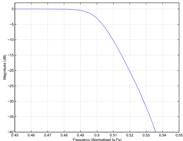
Figure 9-10. Transition Band (Detail)—DAC, F_{s_{int}} = 48.000 kHz
