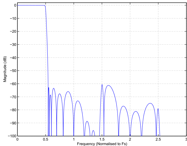
Figure 9-8. Stopband—DAC, F_{s_{int}} = 48.000 kHz
