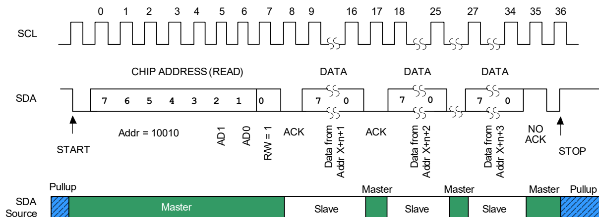
Figure 4-28. Control-Port Timing, I²C Reads with Autoincrement
