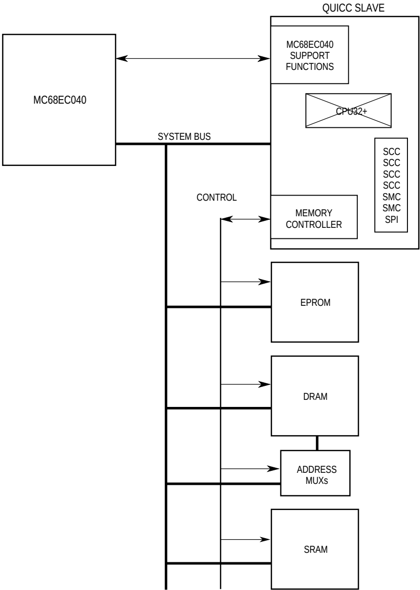
Figure 1-22. MC68040 Companion Mode
