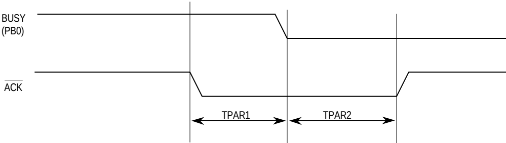
Figure 7-90. Centronics Receiver Timing Mode 1
