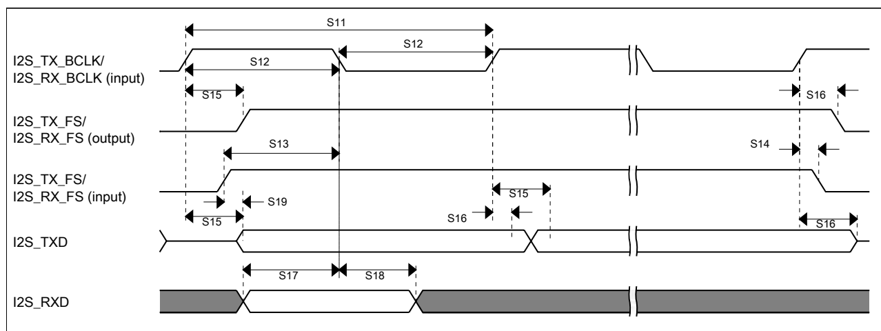
Figure 40. I2S/SAI timing — slave modes
