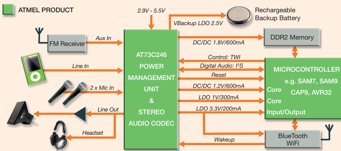
AT73C246 Application Example
