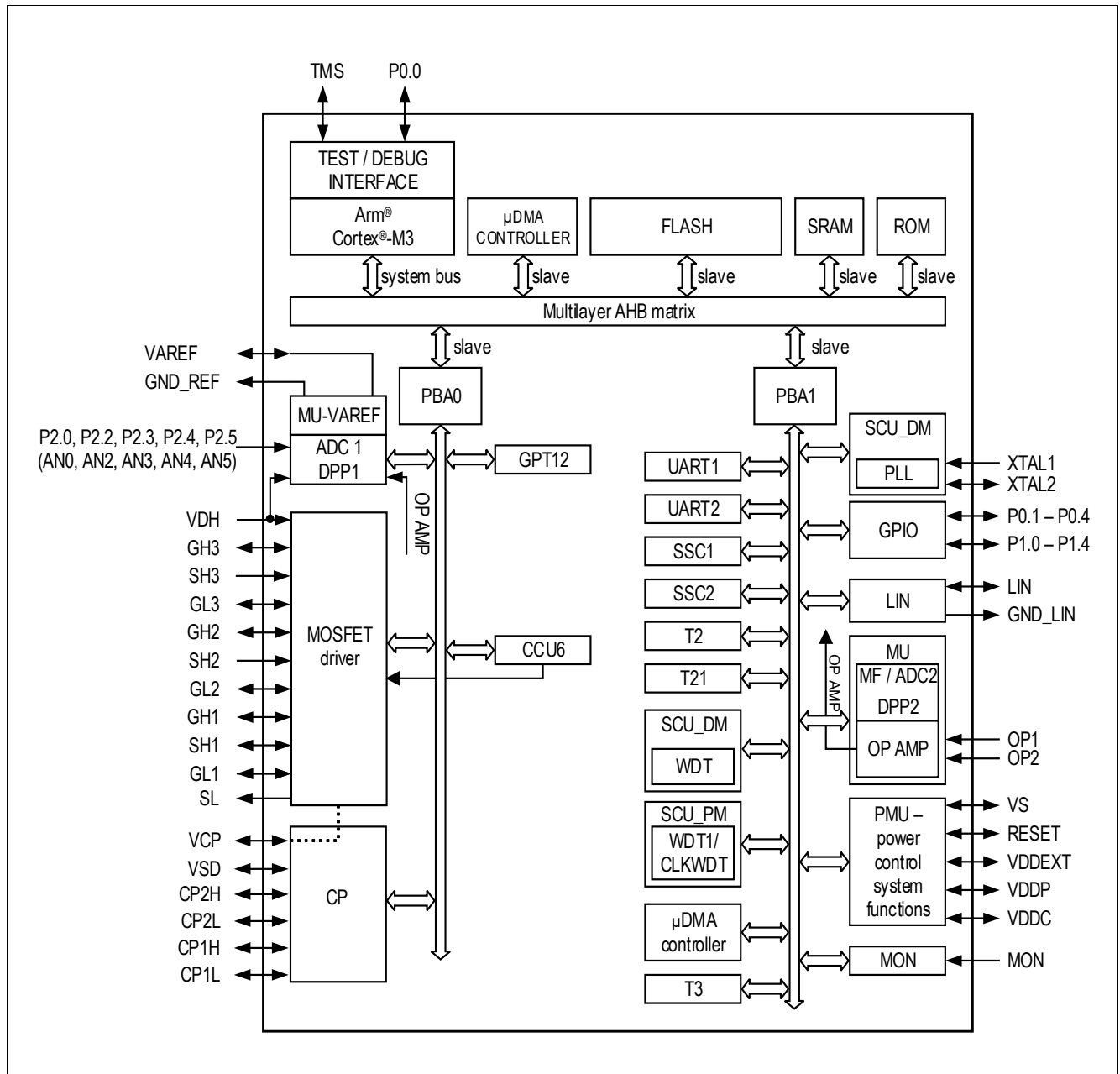
Figure 1 Block diagram
