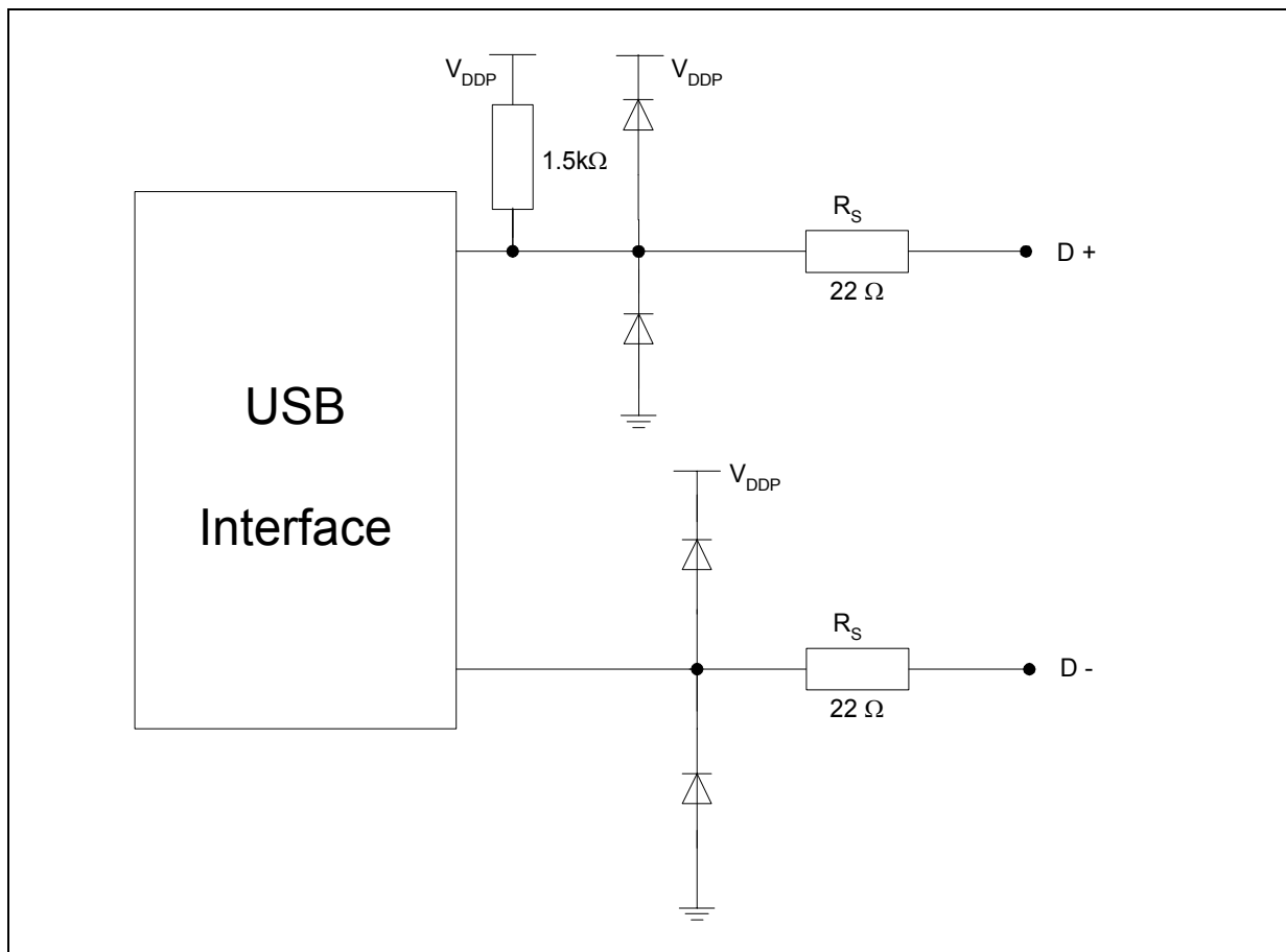
Figure 4-1 USB Interface
