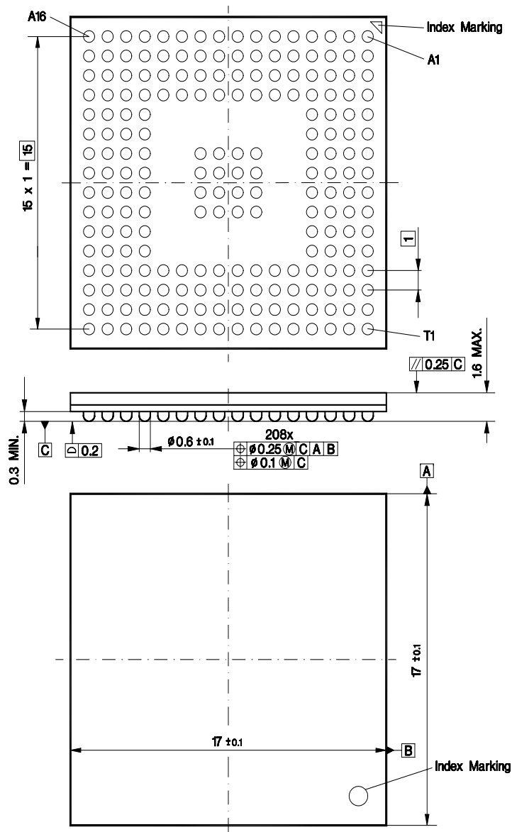
Figure 5-1 P-LBGA-208-2 Package
