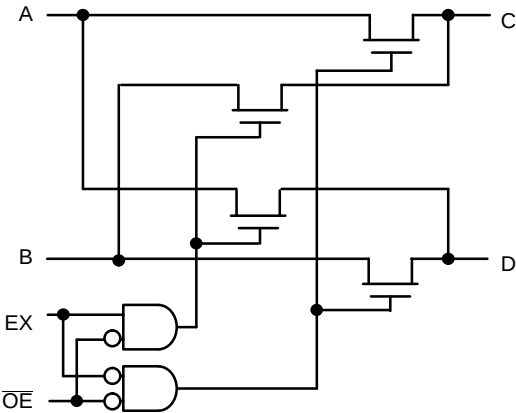
Figure 3. Logic Diagram
