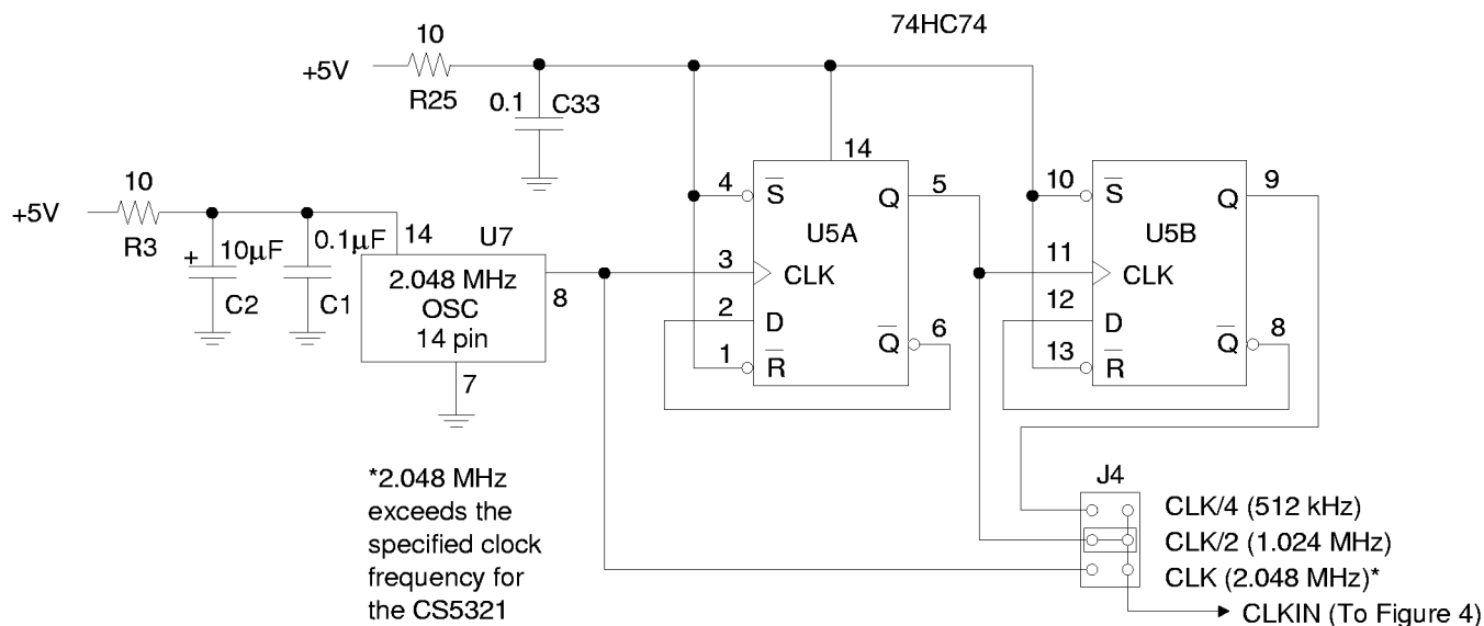
Figure 3. Oscillator / Divider
