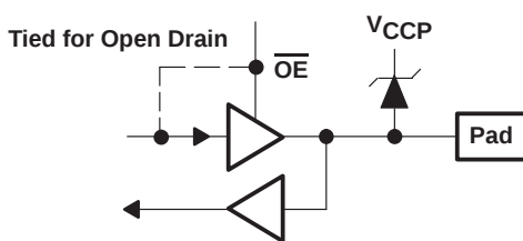
Figure 3–2. 3-State Bidirectional Buffer
