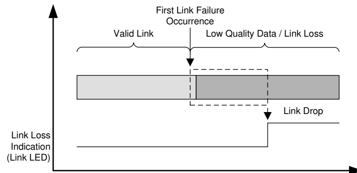
Figure 9-8. Fast Link-Drop
