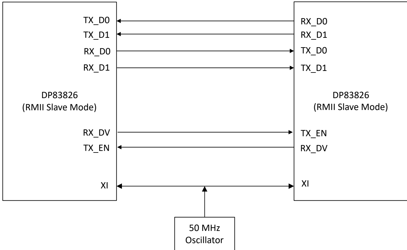
Figure 9-3. RMII Repeater Mode: Slave-Slave
