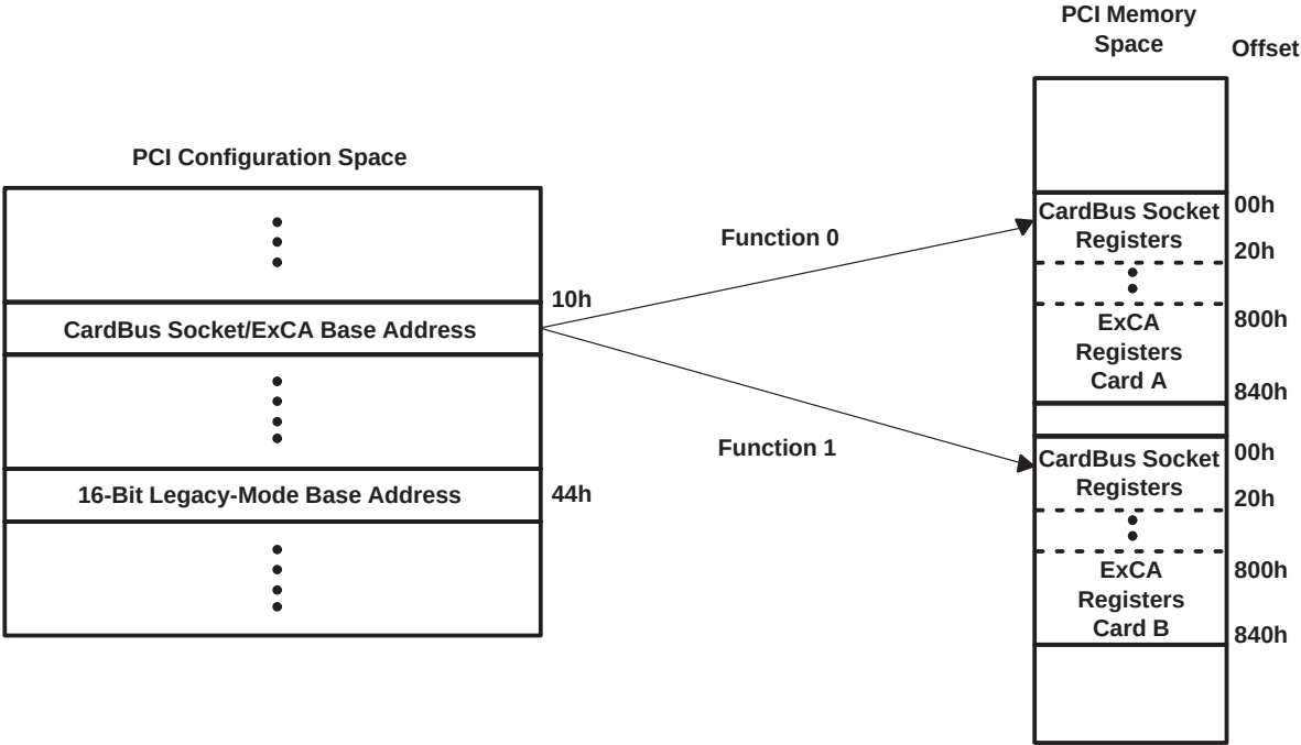
Figure 12. CardBus Socket/ExCA PCI Memory Access Method
