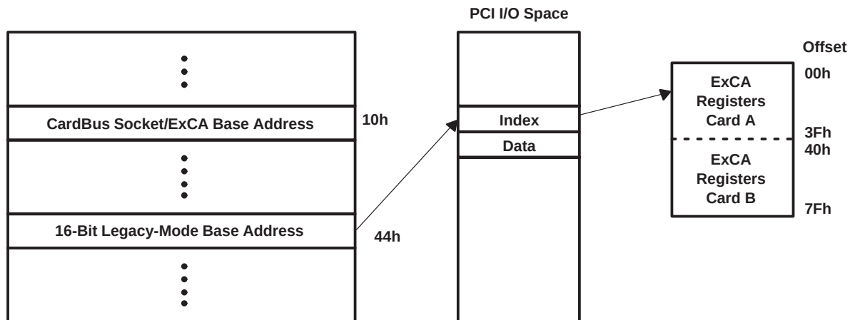
Figure 11. ExCA PCI I/O Legacy Access Method
