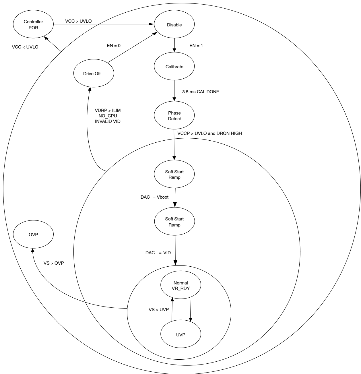
Figure 9. State Diagram
