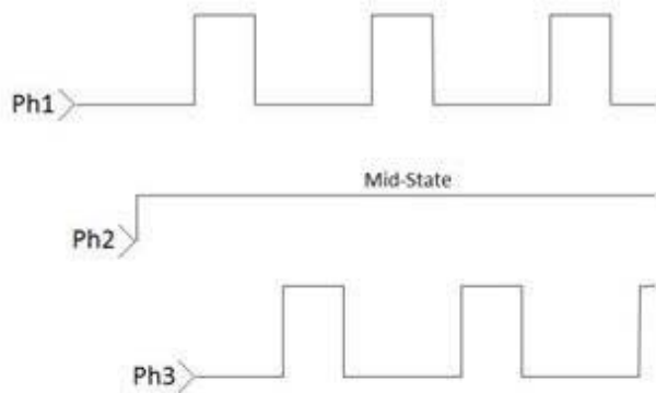
Figure 20. 2 Phase Mode
