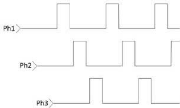
Figure 19. 3 Phase Mode
