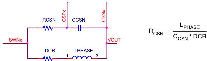
Figure 12. Differential Current Feedback
