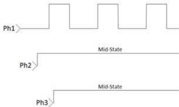
Figure 21. 1 Phase Mode
