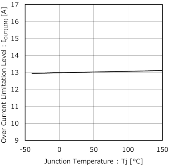
Figure 19. Over Current Limitation Level vs Junction Temperature ( V_{OUT} = 12\text{ V} )
