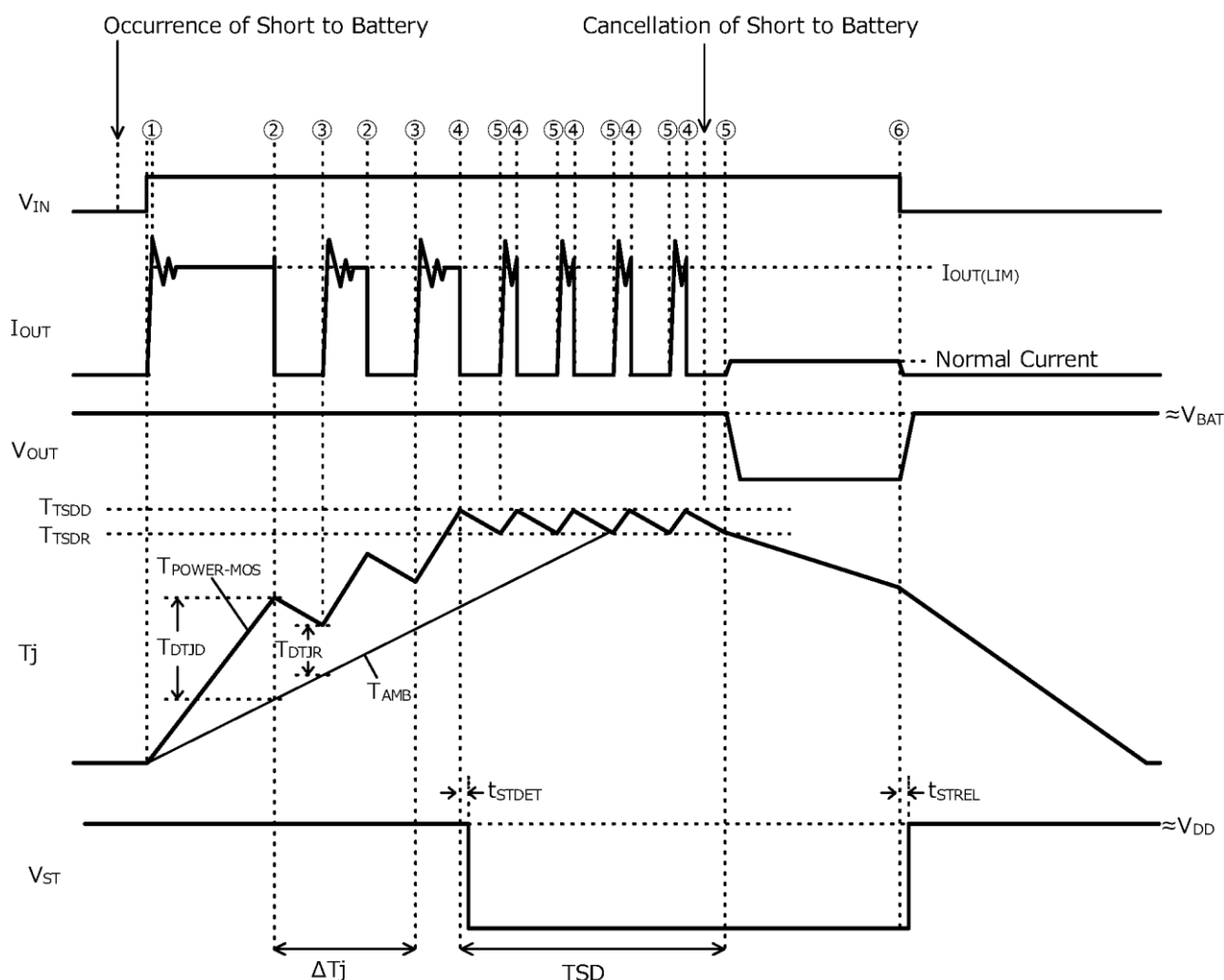
Figure 23. The Behavior when the OUT Pin Short Circuit
