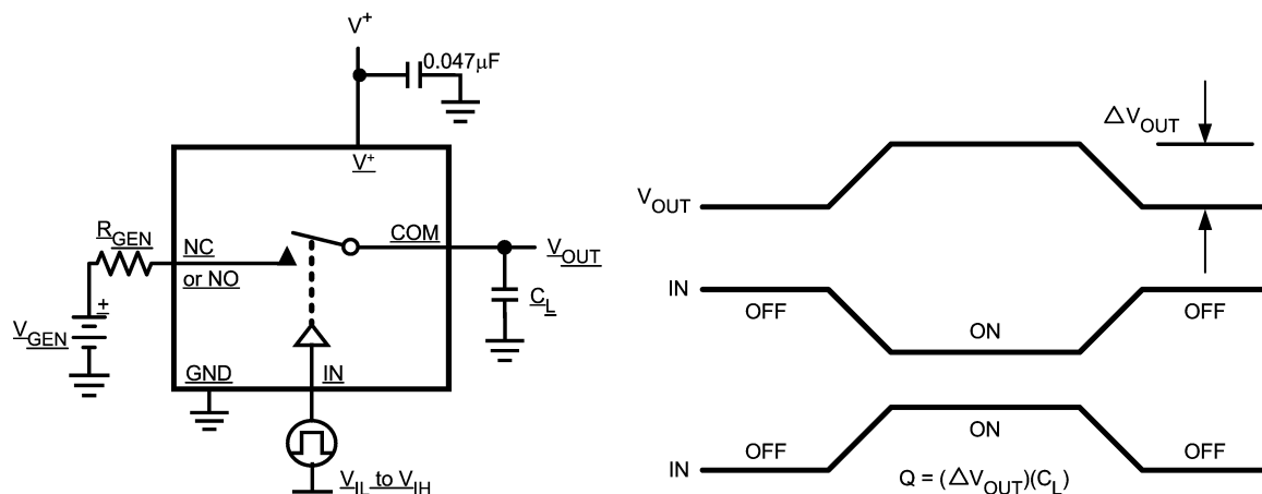
FIGURE 3. Charge Injection
