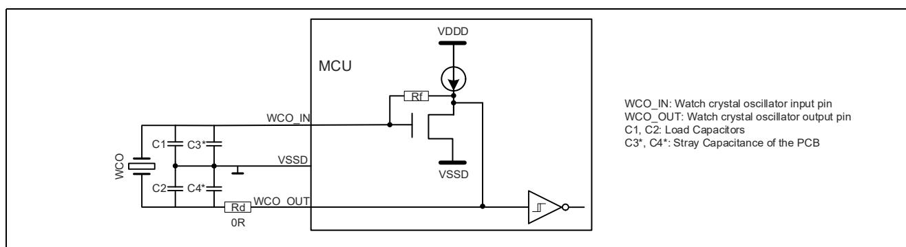
Figure 26-23 WCO connection scheme [72]
