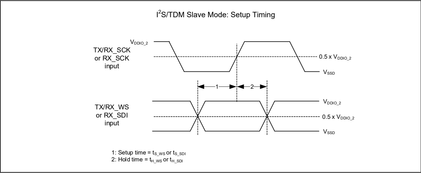
Figure 26-39 Slave setup
