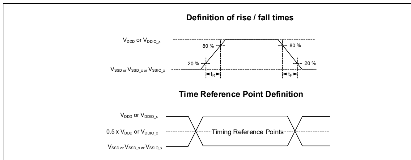
Figure 26-7 AC timings specifications
