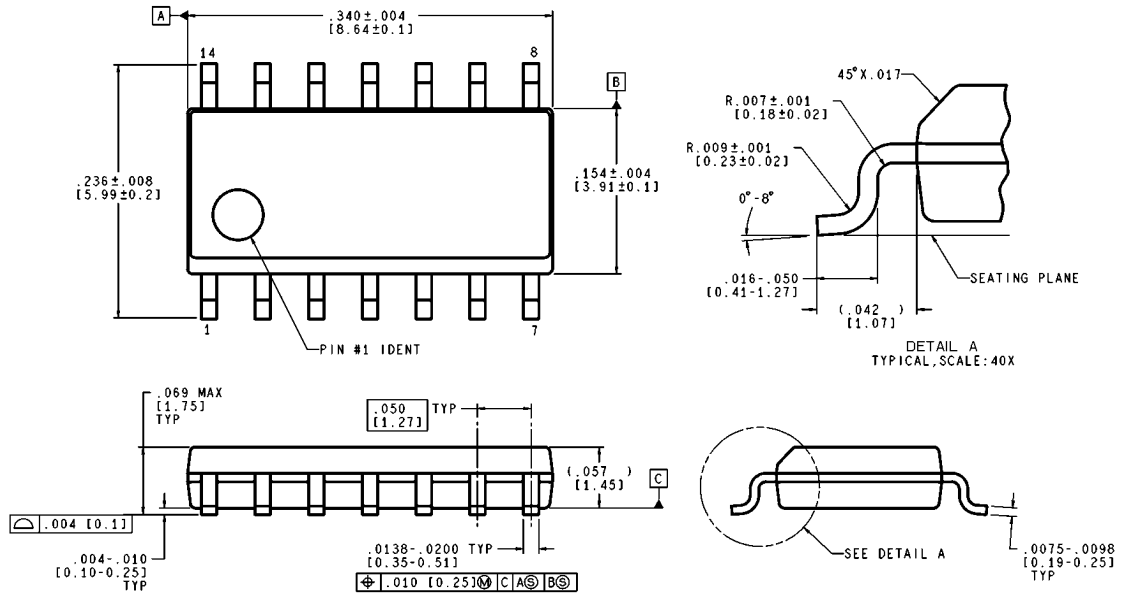
CONTROLLING DIMENSION IS INCH VALUES IN [ ] ARE MILLIMETERS
