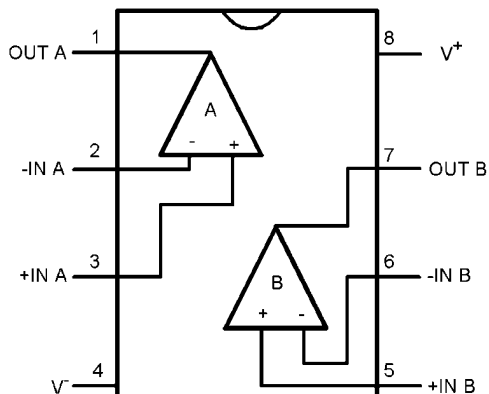
8-Pin SOIC and 8-Pin MSOP (LMH6643)
