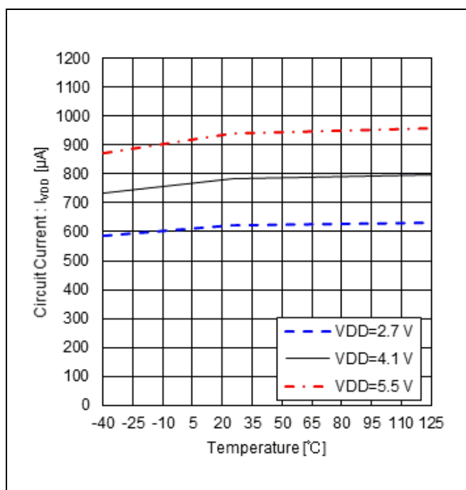
Figure 7. Circuit Current vs Temperature
