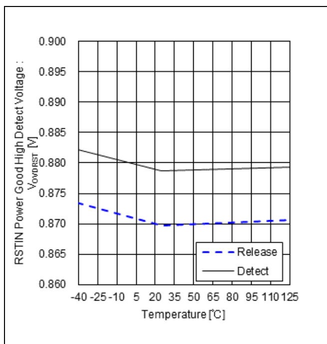
Figure 9. RSTIN Power Good High Detect Voltage vs Temperature ("RSTIN OVD", V_{DD}=3.3 V)
