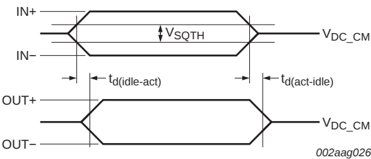
Fig 4. LFPS electrical idle transitions in U0/U1 modes
