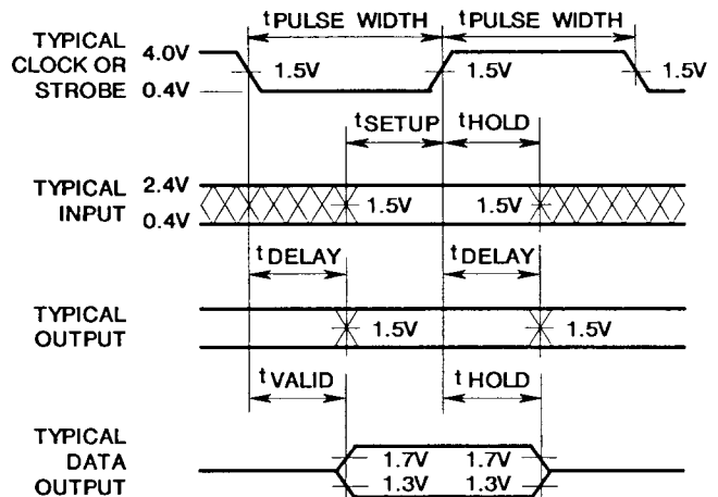
FIGURE 22. A.C. DRIVE AND MEASURE POINTS - CLK INPUT
