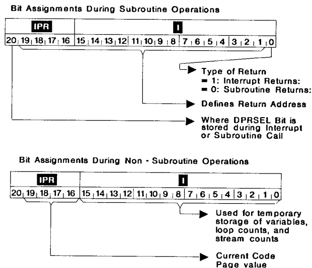
FIGURE 11. I AND IPR BIT ASSIGNMENTS
