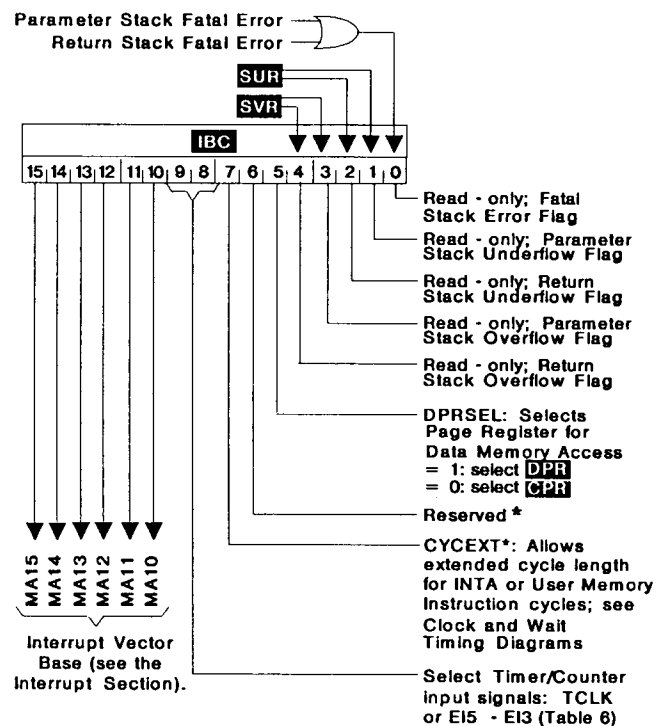
FIGURE 5. IBC BIT ASSIGNMENTS
