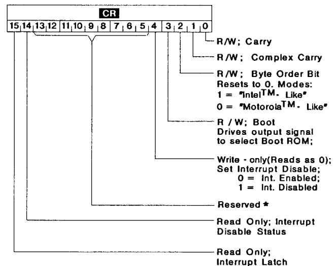
FIGURE 3. CR BIT ASSIGNMENTS
