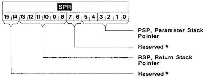
FIGURE 7. SPR BIT ASSIGNMENTS
