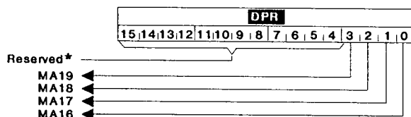
FIGURE 12. DPR BIT ASSIGNMENTS
