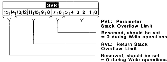
FIGURE 8. SVR BIT ASSIGNMENTS
