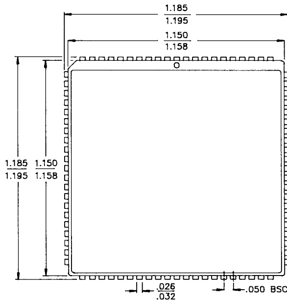
TOP VIEW
