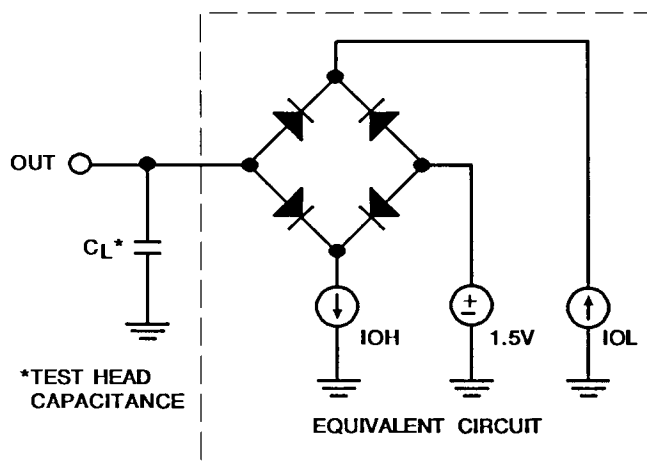
FIGURE 21. TEST CIRCUIT
