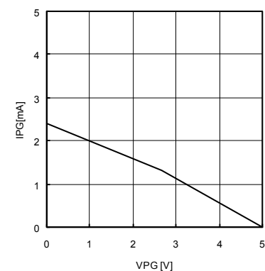
Fig. 6 PG Pin Source Current
