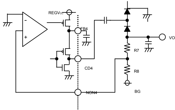
Fig. 31 Low-side Charge Pump Circuit Diagram
