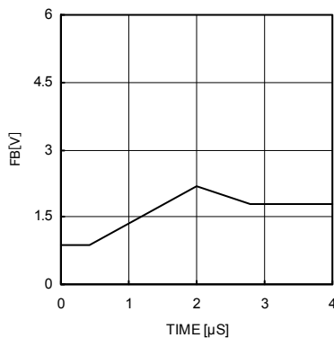
Fig. 8 Error Amp Slew Rate Waveform
