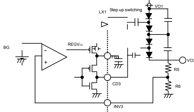
Fig. 30 High-side Charge Pump Circuit Diagram
