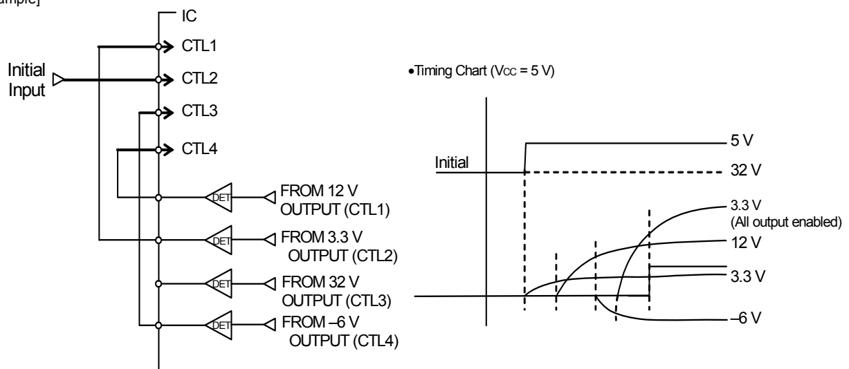
Fig. 38 Timing Chart
