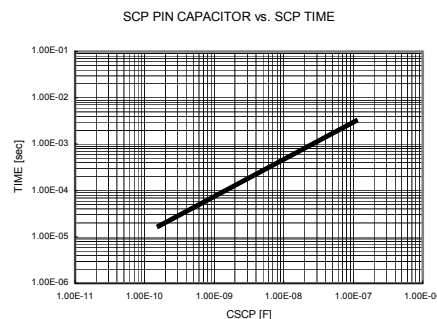
Fig. 29 SCP Capacitance vs Short Protection Delay Time
