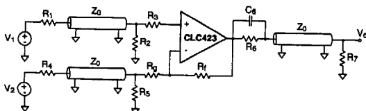
Figure 6: Transmission Line Matching
