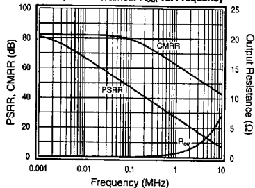
PSRR, CMRR & Linear R_{out} vs. Frequency
