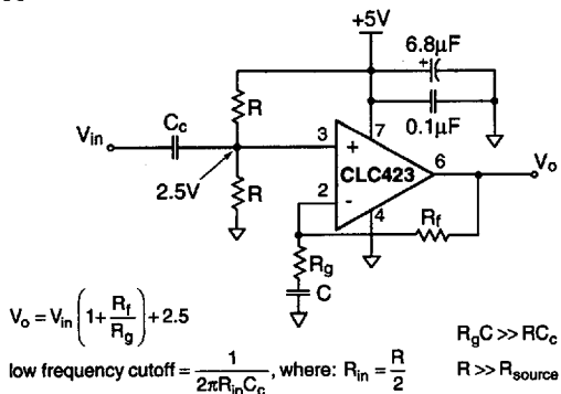
Figure 3: AC Coupled Non-Inverting Configuration
