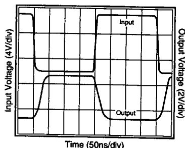
Figure 5: Overdrive Recovery
