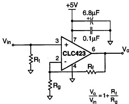
Figure 1: Non-Inverting Configuration
