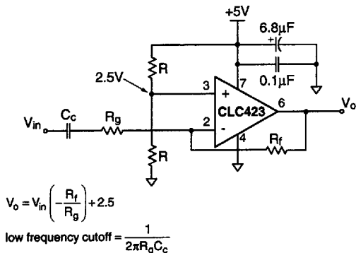
Figure 4: AC Coupled Inverting Configuration
