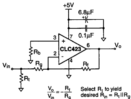
Figure 2: Inverting Configuration
