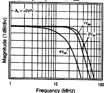
Frequency Response vs. V_{out}
