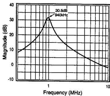
Figure 10: Bandpass Response
