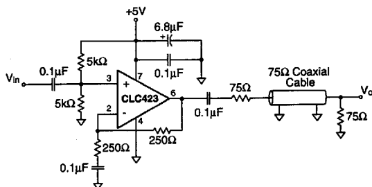
Figure 8: Single Supply Cable Driver
