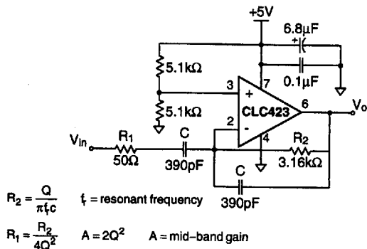
Figure 9: Bandpass Filter Topology
