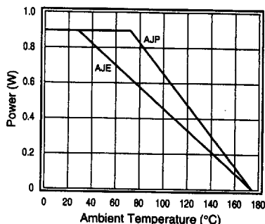
Figure 7: Power Derating Curves
