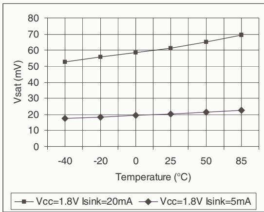
Figure 6. V_{SAT} vs. temperature
