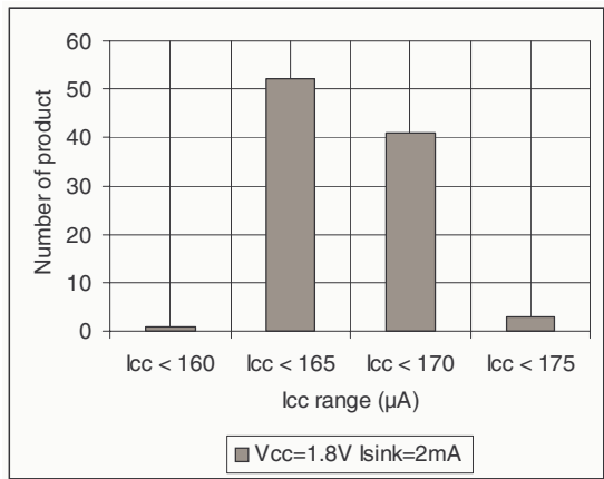
Figure 5. I_{CC} at 25 ^{\circ} C
