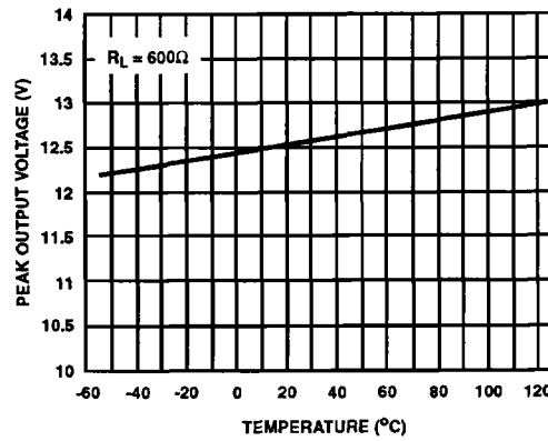
FIGURE 14. OUTPUT VOLTAGE SWING vs TEMPERATURE
