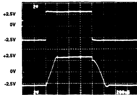
FIGURE 2. LARGE SIGNAL RESPONSE
