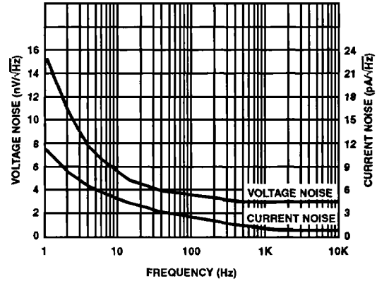
FIGURE 20. NOISE CHARACTERISTICS
