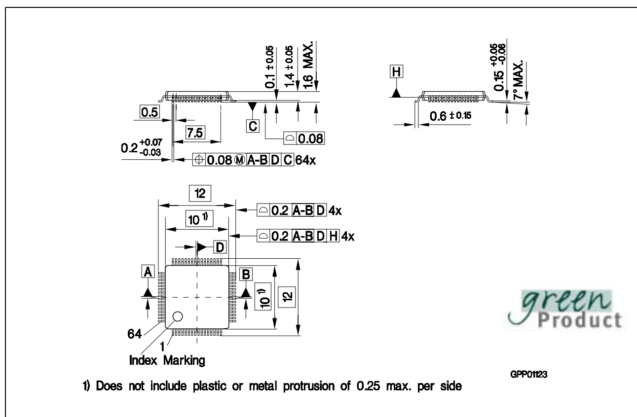
Figure 16 PG-LQFP-64-4 (Plastic Green Low Profile Quad Flat Package), valid for the -16F derivatives
