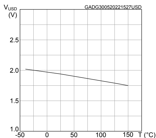
Figure 21. Undervoltage shutdown
