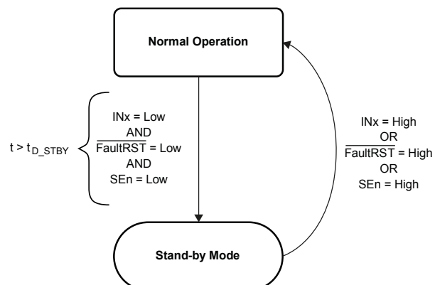
Figure 11. Standby state diagram
