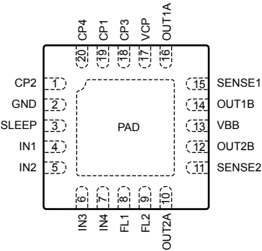
PINOUT DIAGRAM
