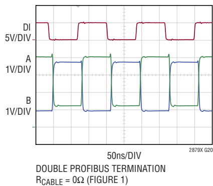
PROFIBUS Operation at 12Mbps V_{CC} = 5\text{V}
