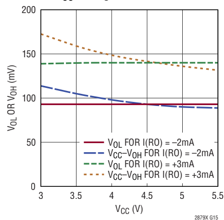
Receiver Output Voltage vs V_{CC} Voltage
